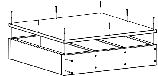
FRAMED FLOOR RISER CONSTRUCT A FLOOR SUPPORT FRAME (MINIMUM 36 INCHES [92CM] SQUARE) FROM PRESSURE TREATED LUMBER OF 2 IN [50MM] NOMINAL THICKNESS AND OF THE DESIRED HEIGHT. SPACE FRAME MEMBERS NO MORE THAN 10 IN [25CM] APART. COVER THIS STRUCTURE WITH PRESSURE TREATED PLYWOOD. SECURE ALL JOINTS WITH CORROSION RESISTANT SCREWS.
