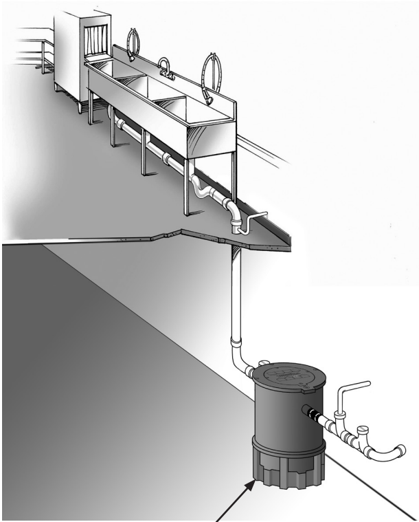
SSOP-70/95, SSA-27 Support Stand for TSS-70, TSS-95, and TSS-27 models Allows unit to be installed directly on the floor in a basement or mechanical room. *Included with -SSA Models
